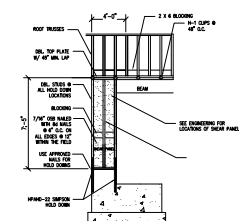
TYPICAL SHEAR WALL < 2/1 RATIO GARAGE DOOR
