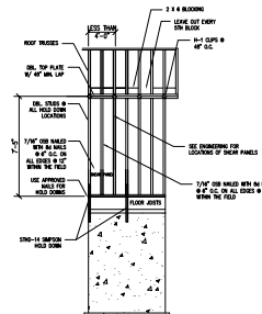
TYPICAL SHEAR WALL 2/1 RATIO
