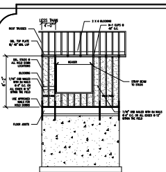
SHEAR TRANSFER THROUGH WINDOW
